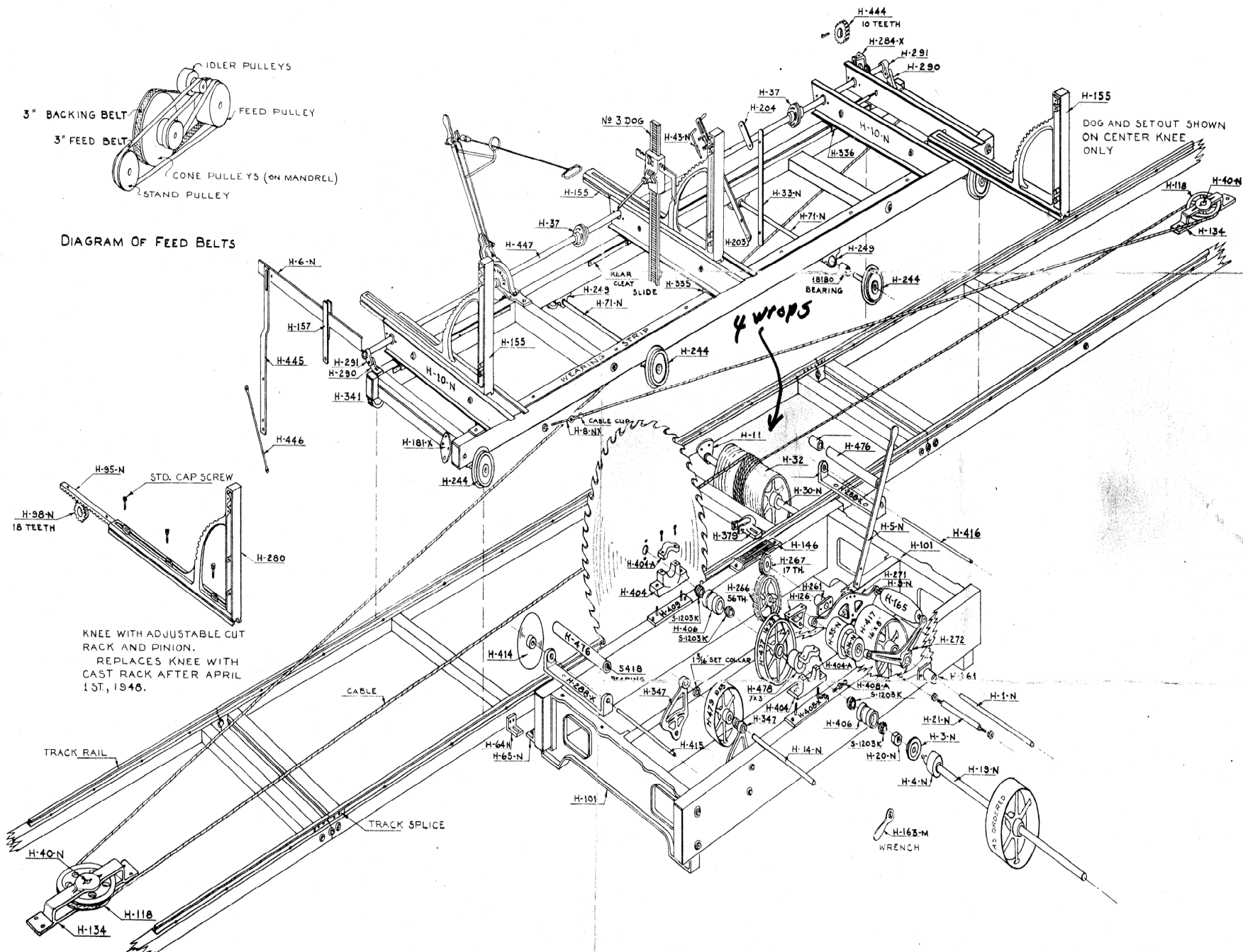
VANCE NO. 100 SAWMILL
