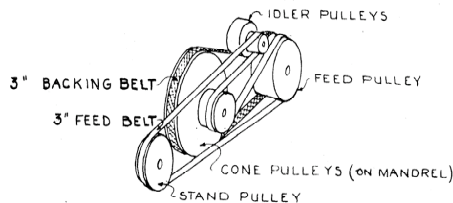
DIAGRAM OF FEED BELTS
